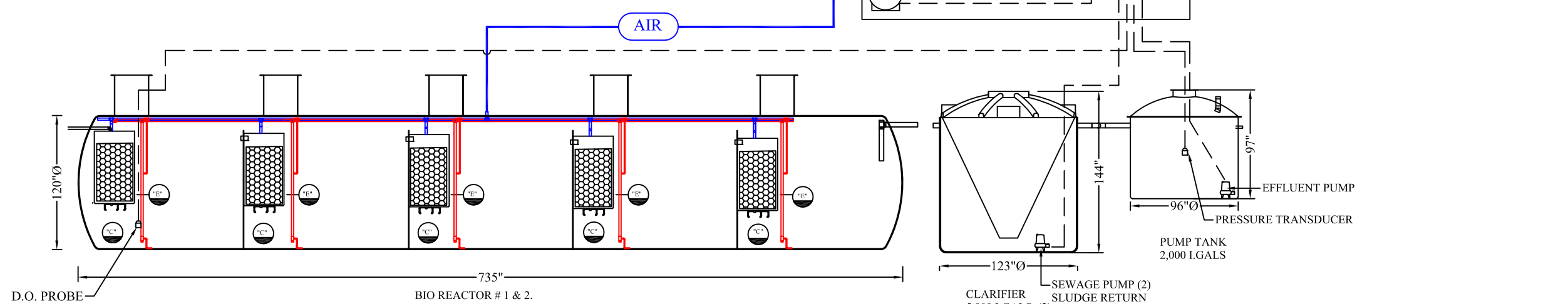
BIO REACTOR # 1 & 2. TREATMENT CAPACITY= 350M 3
