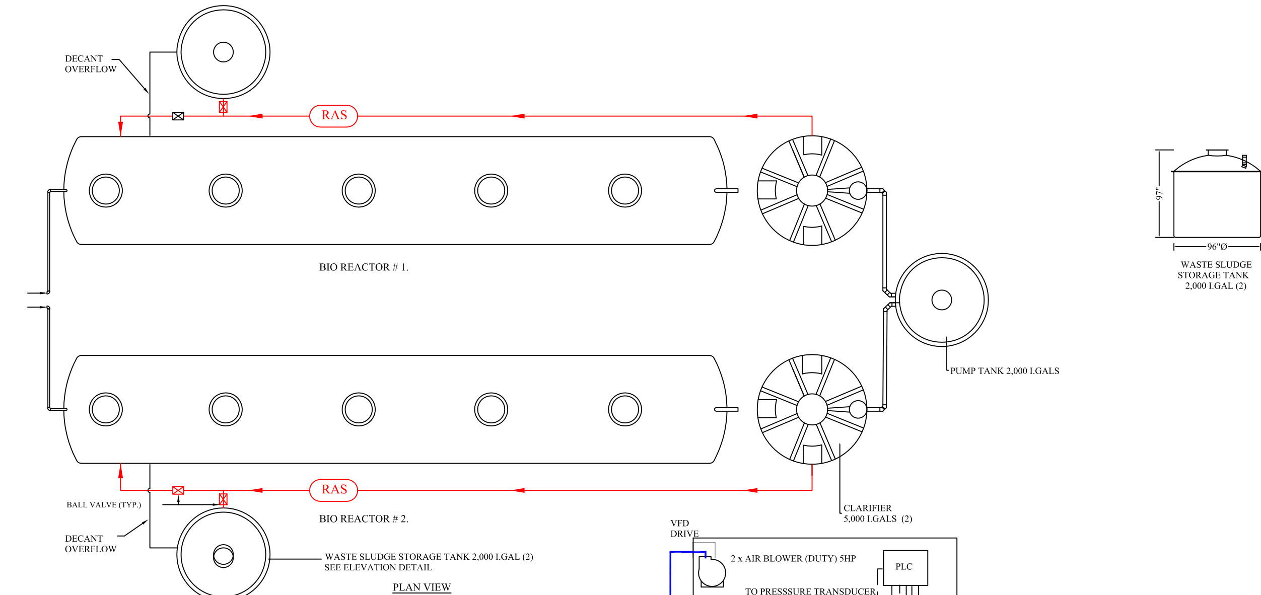
PLAN VIEW
