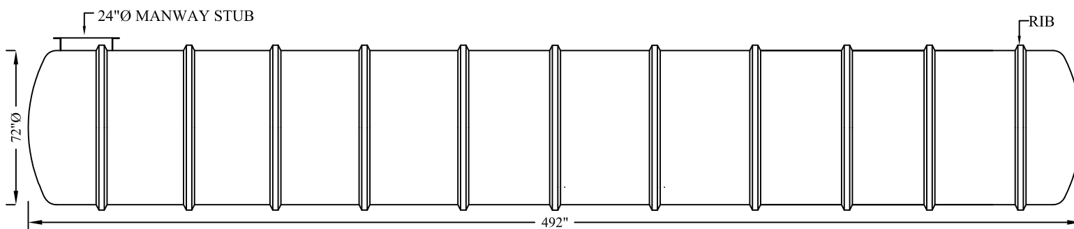
ELEVATION VIEW
