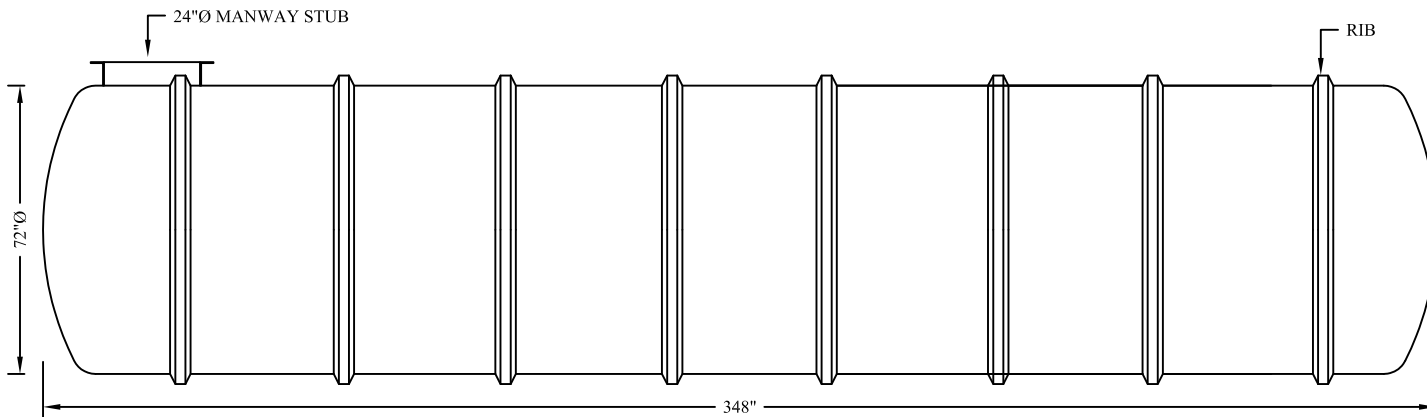
ELEVATION VIEW
