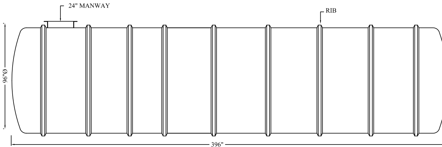
ELEVATION VIEW
