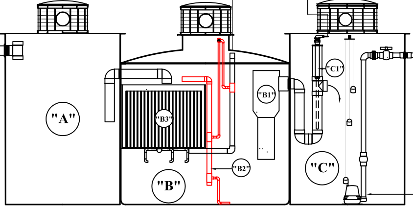
ELEVATION-SECTION
