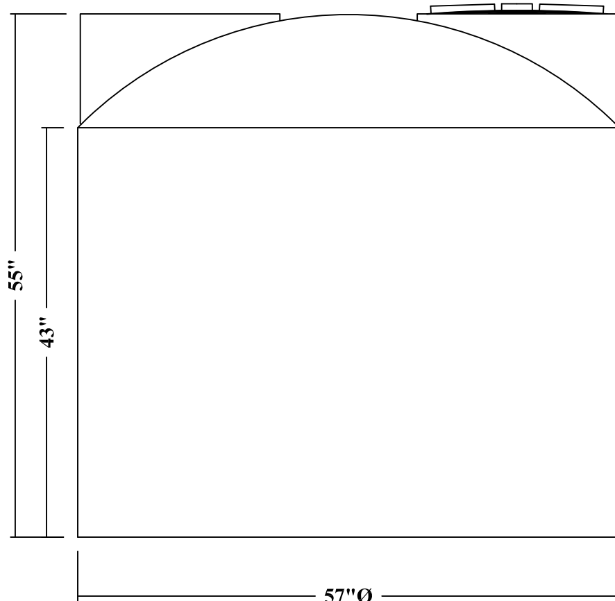
ELEVATIONS
