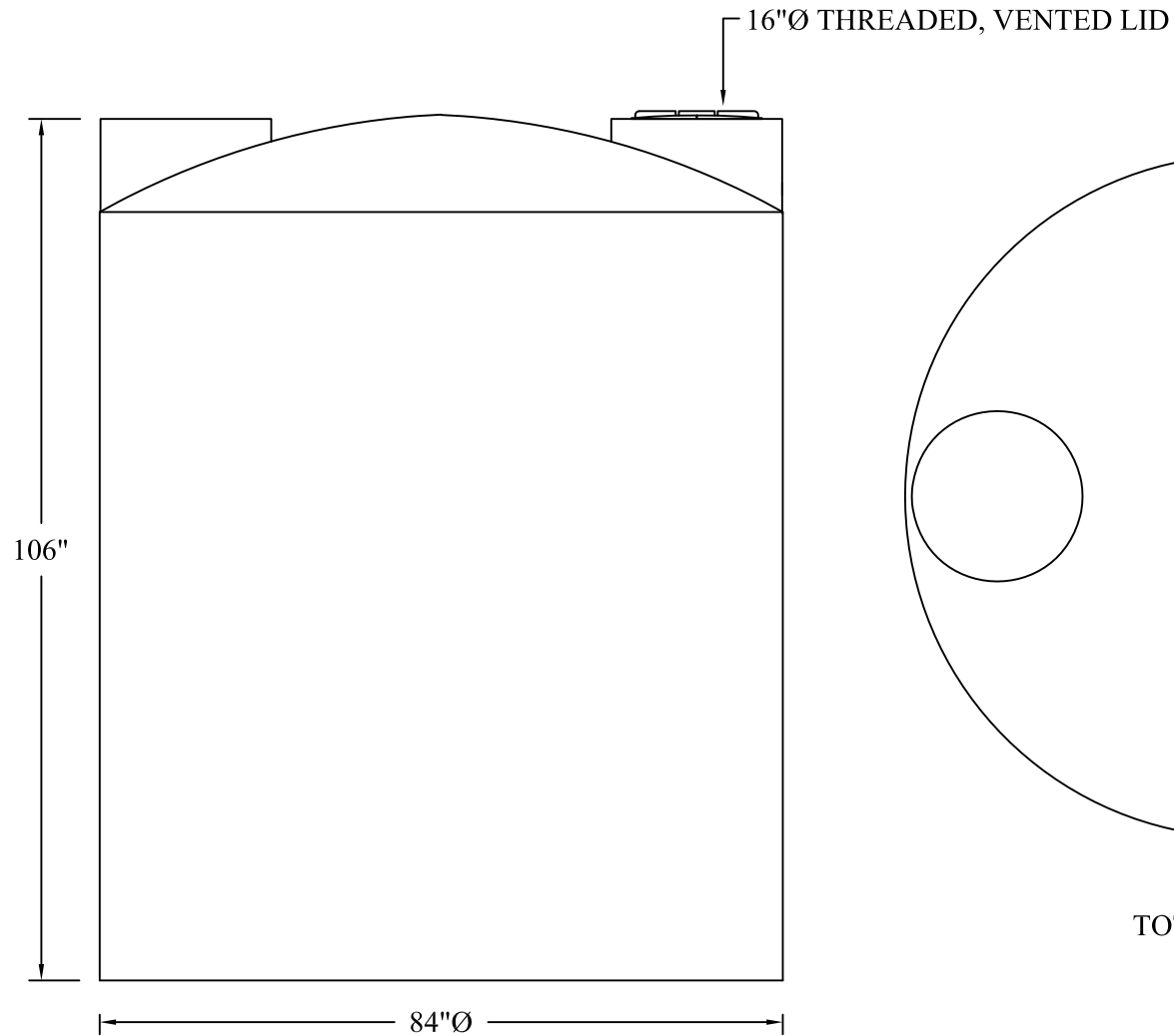
ELEVATION HD;PE POLLYETHYLENE STORAGE TANK MODLE RK2000
