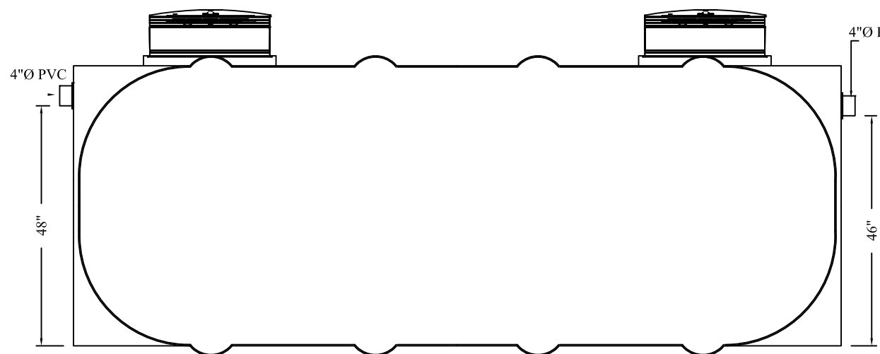
1,400 I.GALS TRASH TANK DIMS.: 58" X 154" X 56" H.
