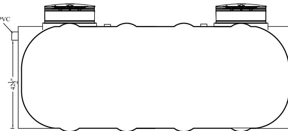
1,000 I. Gals. PUMP / UV CHAMBER DIMS.: 50" X 132" X 53" H. IF REQUIRED
