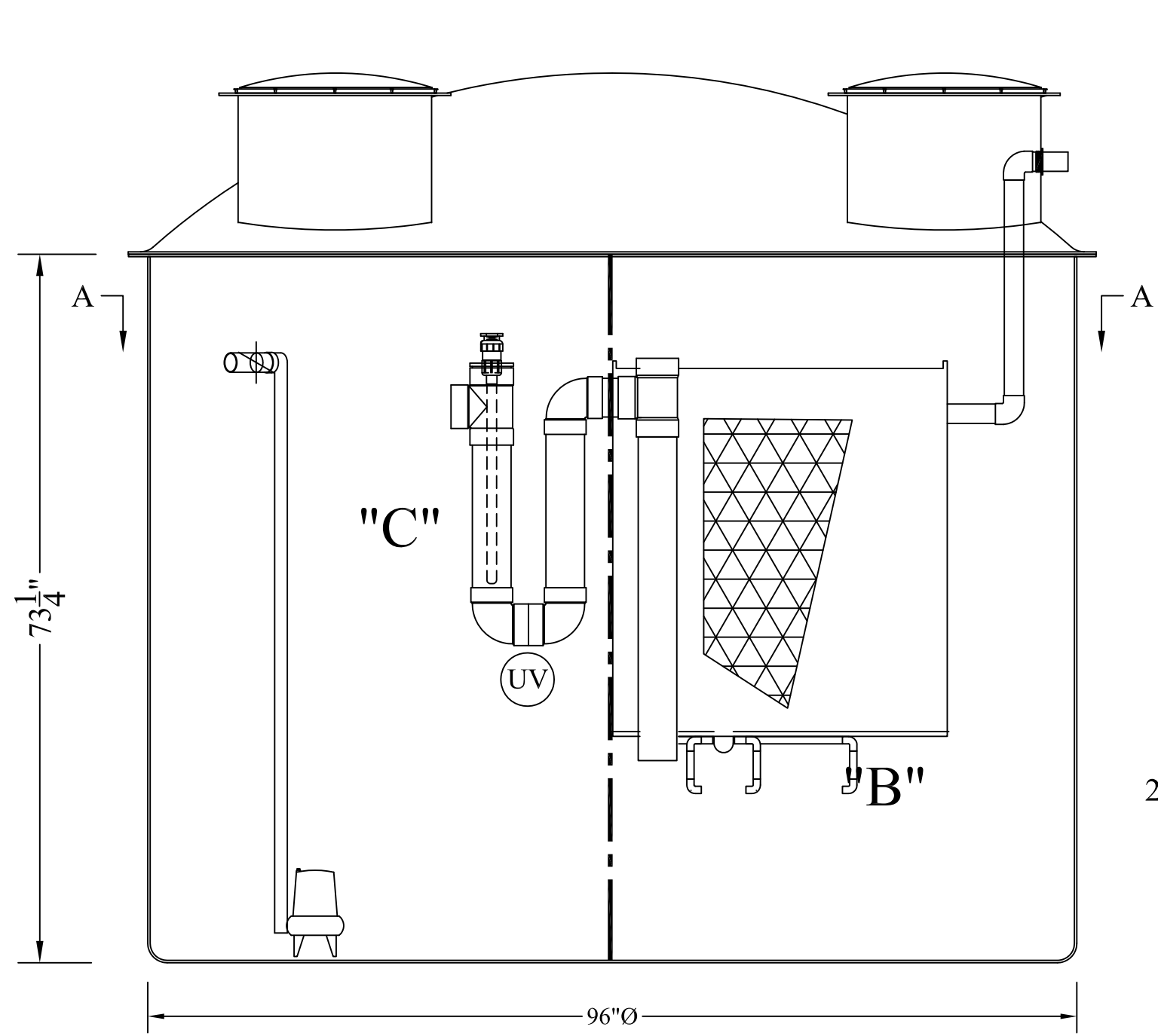
COMPACT ECOPOD MODEL ECOPOD E75-3-T3-COMPACT
