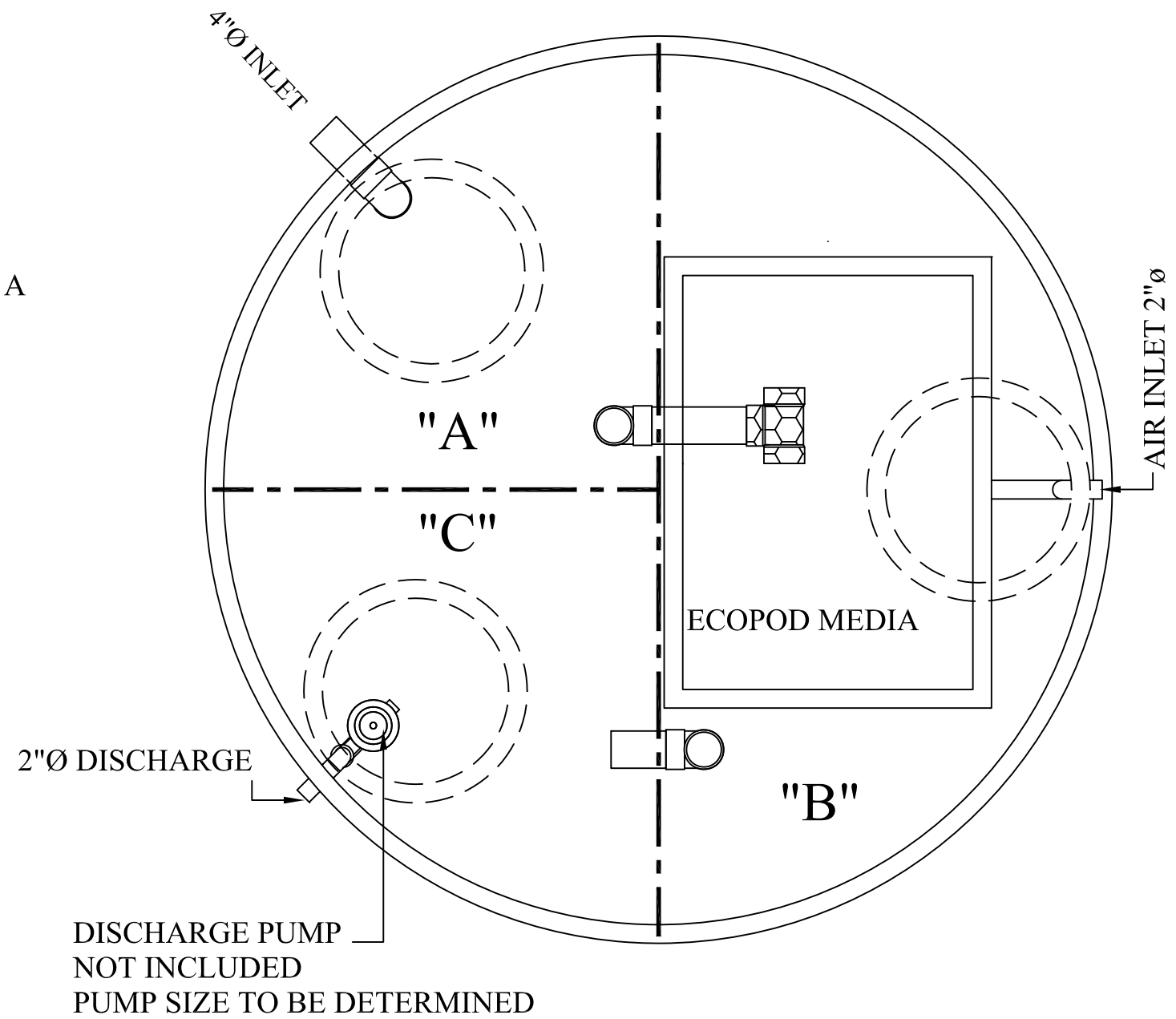
TOP VIEW LID OFF A-A
