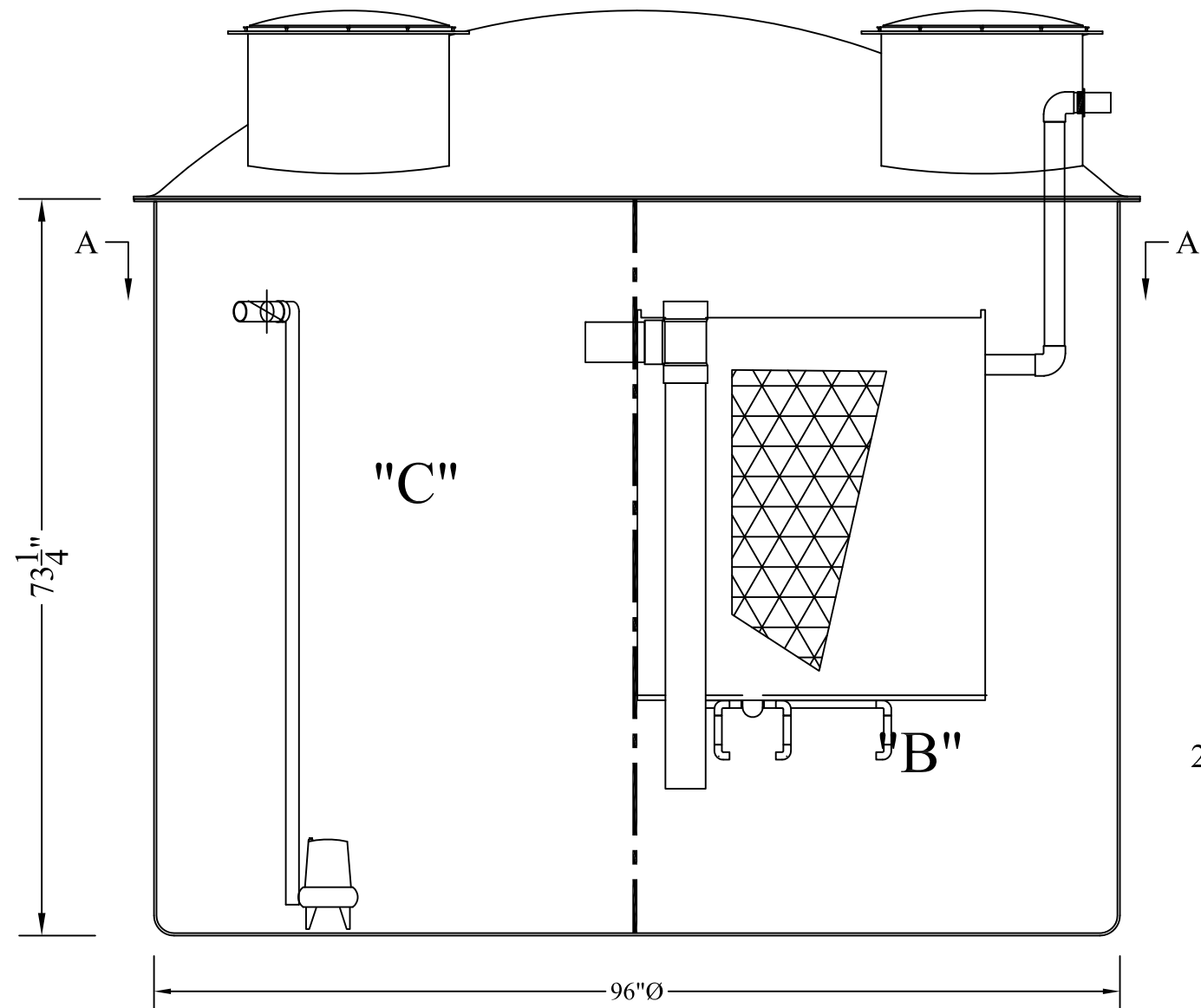
COMPACT ECOPOD MODEL ECOPOD E75-3-T2-COMPACT
