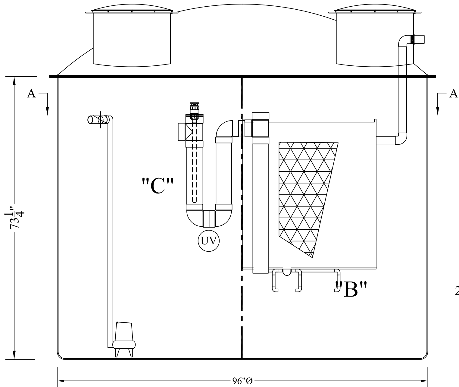
COMPACT ECOPOD MODEL ECOPOD E60-3-T3-COMPACT
