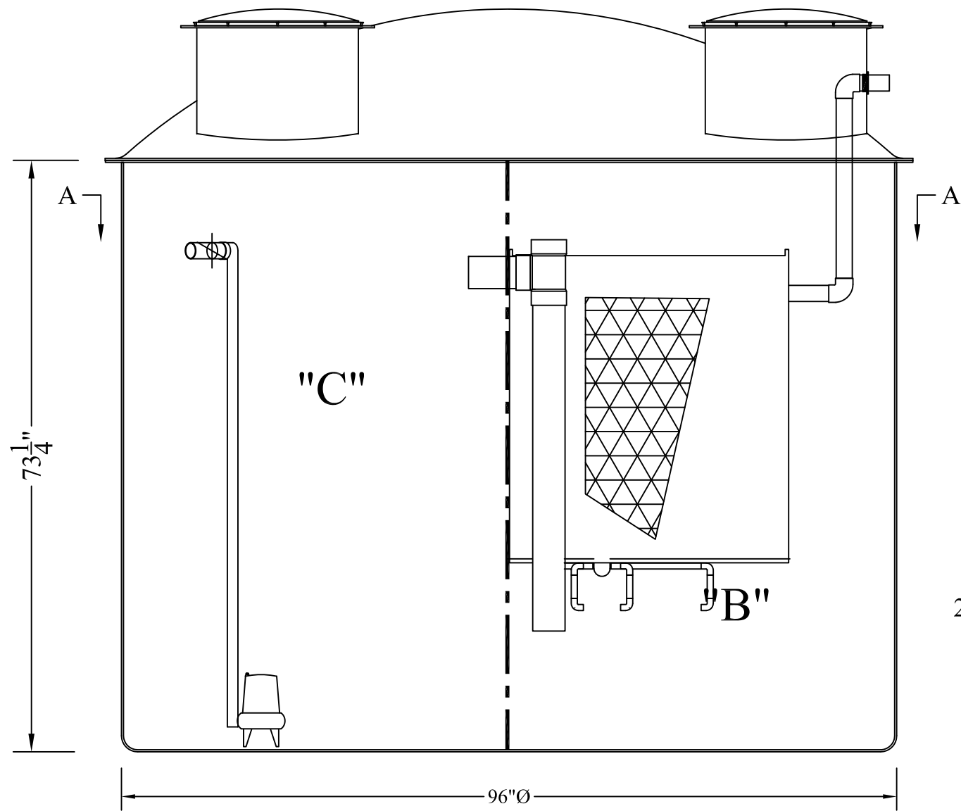
COMPACT ECOPOD MODEL ECOPOD E60-3-T2-COMPACT
