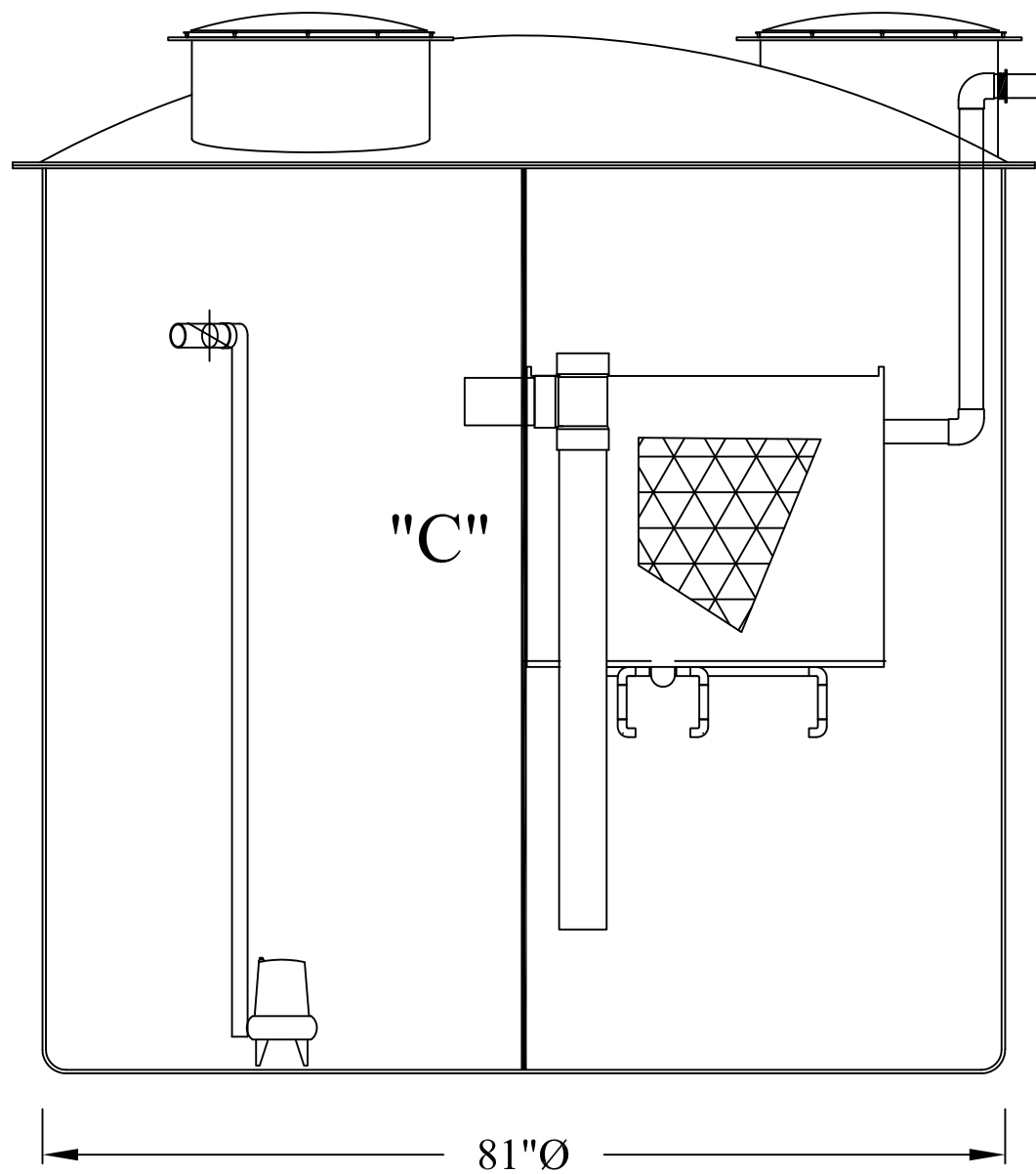
COMPACT ECOPOD MODEL ECOPOD E50-3-T2-COMPACT
