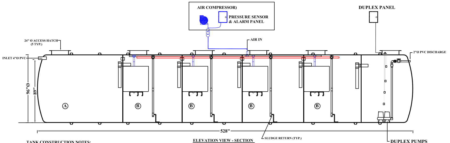
ELEVATION VIEW - SECTION
