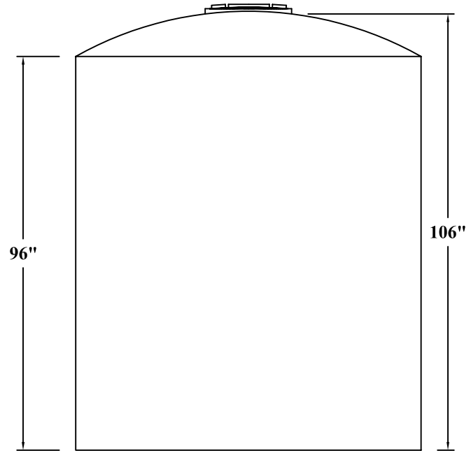
ELEVATION - EAST-WEST
