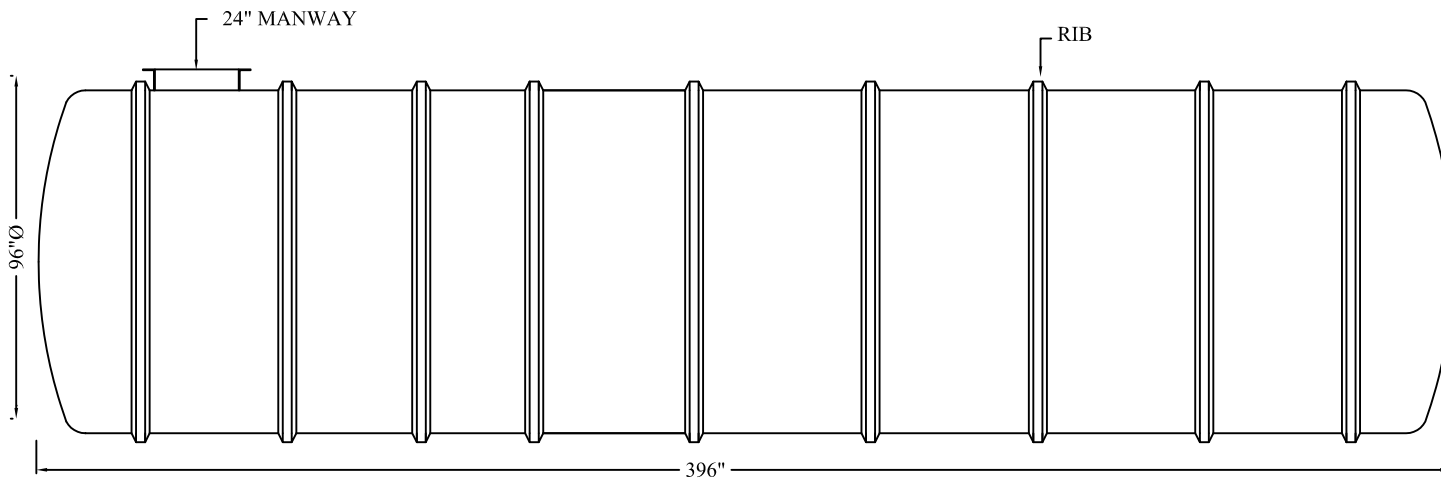
ELEVATION VIEW
