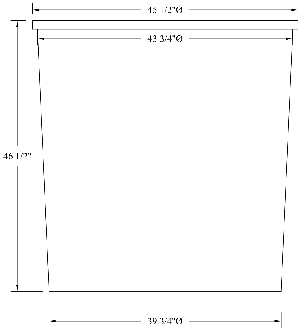
MODEL RKOT200 OPEN TOP TANK CAPACITY: 200 I.GALS 910 L.
