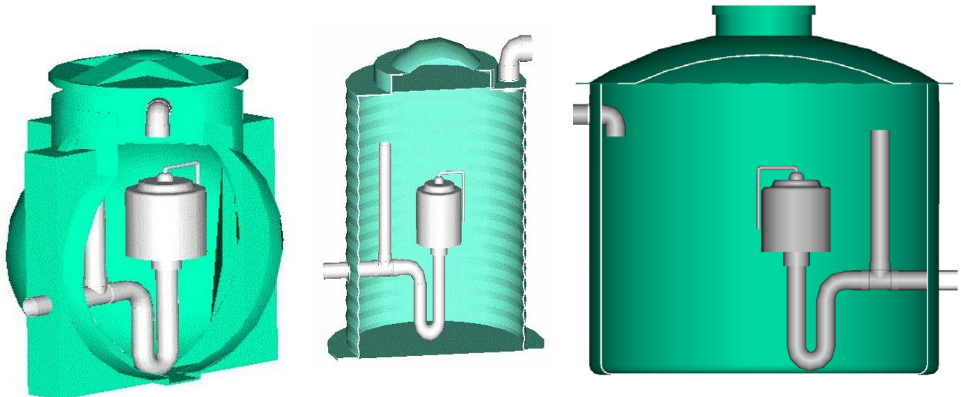
TYPICAL SIPHON INSTALLATION
