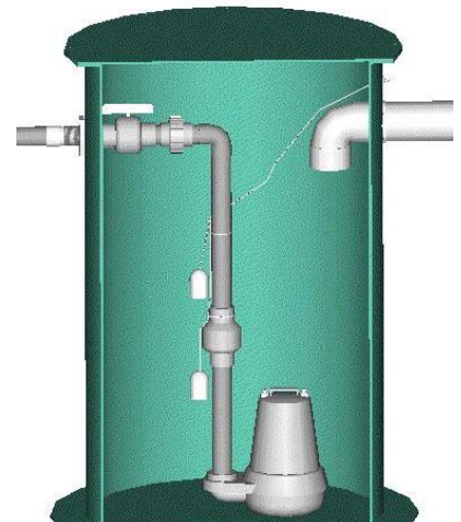
TYPICAL PUMP CHAMBER W/ PUMP INSTALLED
