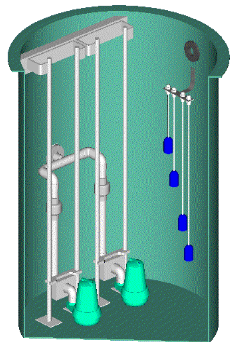
TYPICAL PUMP CHAMBER W/ DUAL PUMPS & PULL-OUT RAIL ASSEMBLY INSTALLED
